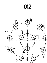
Contact configuration for polarity A (View from B)
