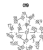
Contact configuration for polarity A (View from B)
