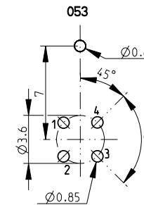
Pin layout / PCB hole pattern for polarity A - View from F (3)
