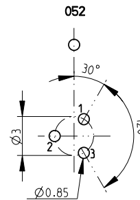
Polarity Z - View from F
