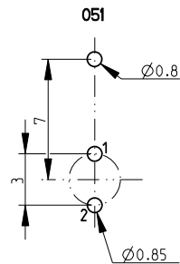
Pin layout / PCB hole pattern for polarity A - View from F (3)
