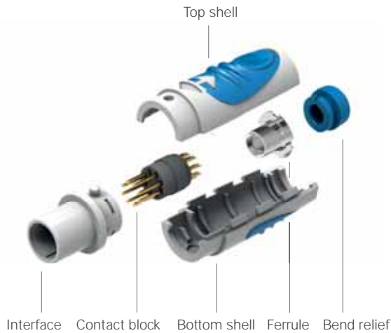
Interface Contact block Top shell Bottom shell Ferrule Bend relief
